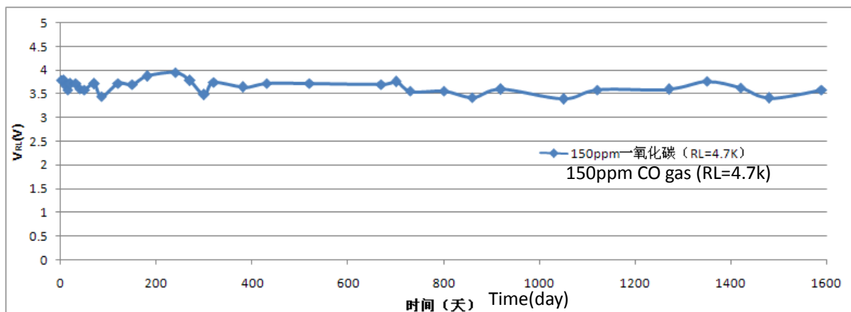
Fig7.long-term Stability
