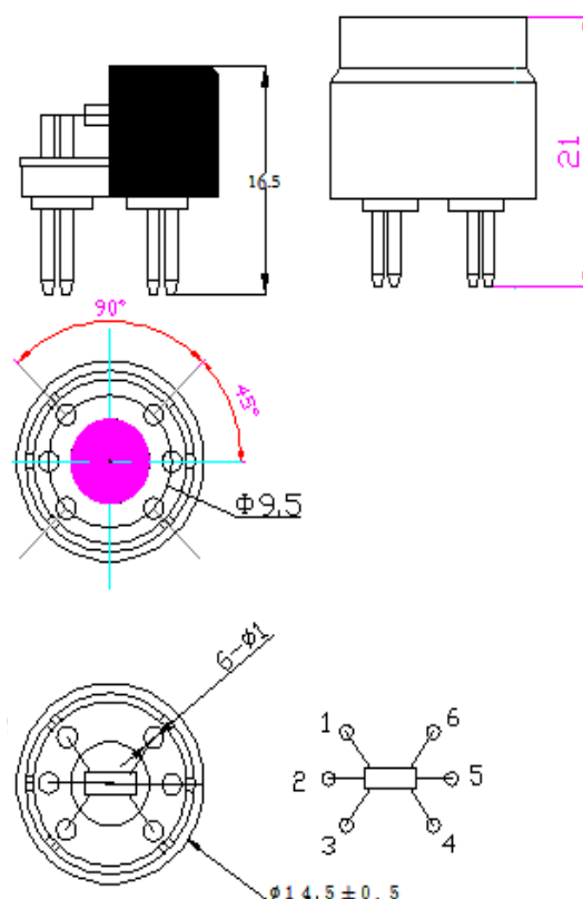
Fig1. Sensor Structure
